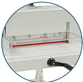
Safety Cover & Back Gauge Crank Plexi cover for safety and spindle guided back gauge for accuracy
